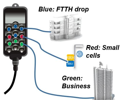
Figure 16: Drop cable terminal interconnect
